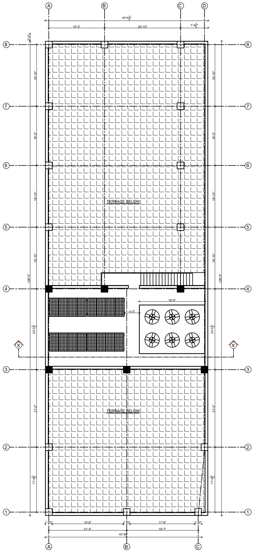
ROOF PLAN
