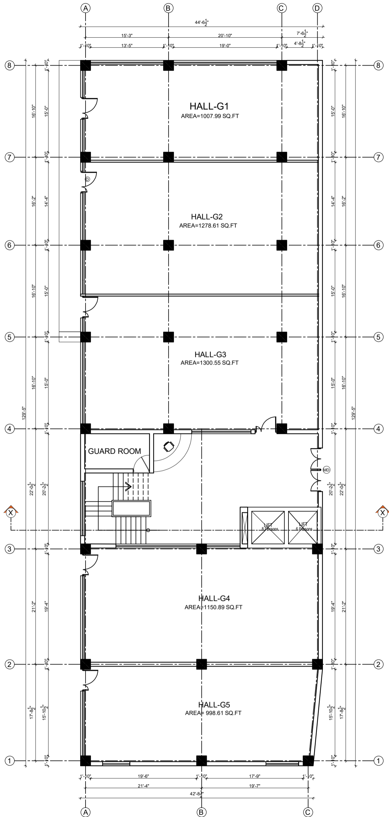
GROUND FLOOR PLAN AREA=5737 SQ.FT
