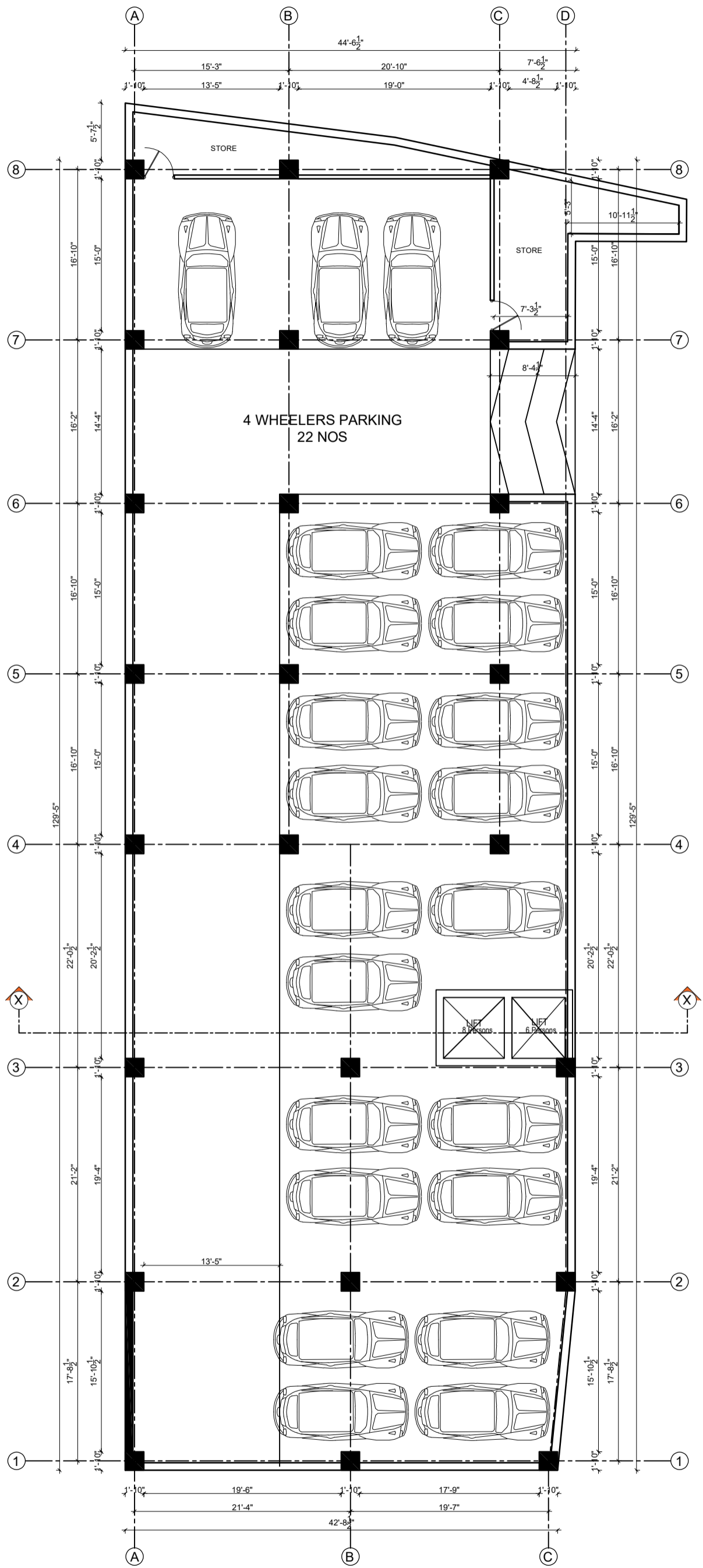
BASEMENT FLOOR PLAN AREA=6000 SQ.FT
