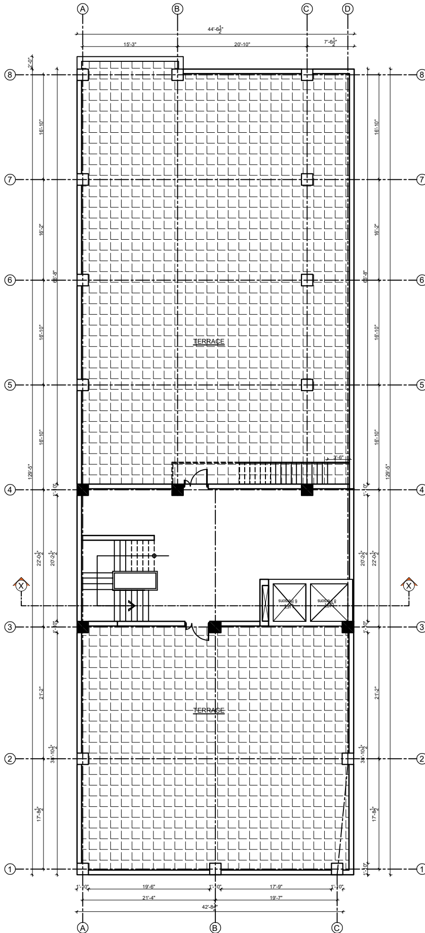
TOP FLOOR PLAN AREA=1063 SQ.FT
